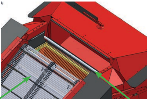
Option chain interval 11mm Hopper Equalizer Option
