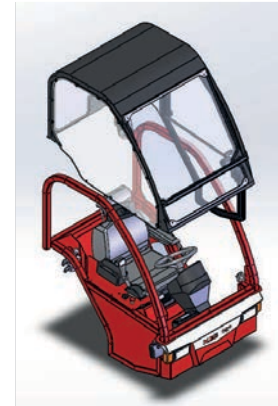
Option Cabin closed
